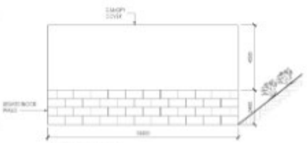
SIDE ELEVATION 1:50
