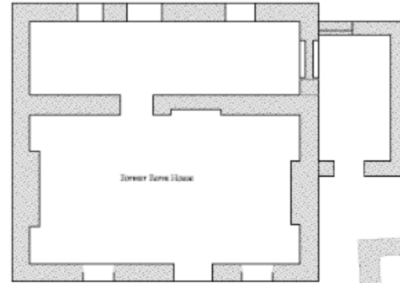
Floor Plan 1/20
